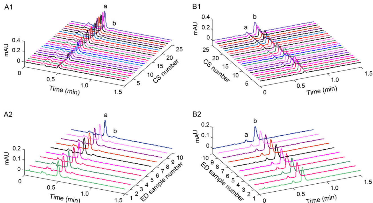
Figure 3. The representative UPLC chromatograms of the calibration set consisting of the 25 run samples (A1 and B1) and the commercial eye drop samples (A2 and B2) (a) BRI and (b) TIM.
