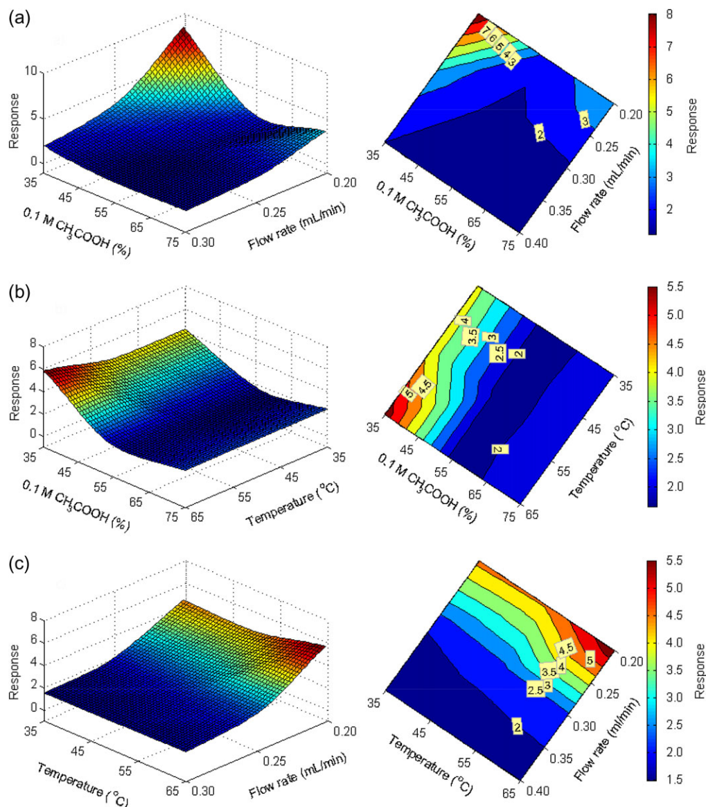
Figure 2. Response surfaces and corresponding contour maps as functions of two factors: flow rate–0.1 M \text{CH}_3\text{COOH} vs. ICRF (a), temperature–0.1 M \text{CH}_3\text{COOH} vs. ICRF (b), flow rate–temperature vs. ICRF (c).
