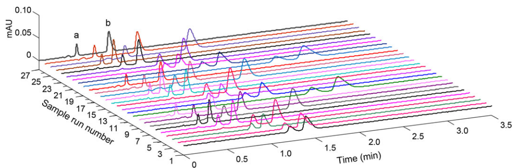
Figure 1. Three-dimensional illustration of the UPLC chromatograms of the 27 run samples, which correspond to the 3^3 full factorial design matrix (a) BRI and (b) TIM.
