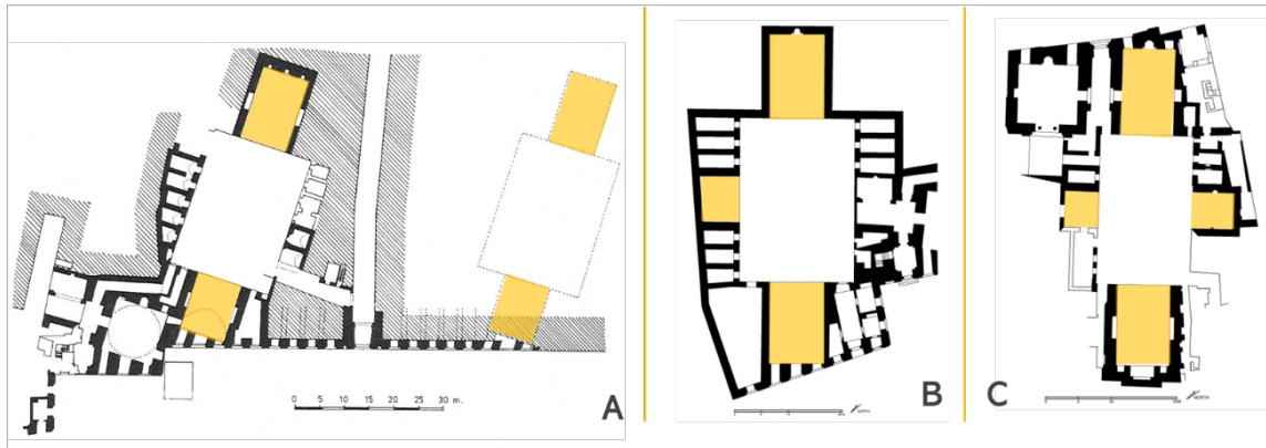
Şekil 2.92. Kahire Salahiye Medresesi (A) (Behrens-Abouseif, 1998: 90), Baybars Zahirîye Medresesi (B) (Arida, 2003e) ve Nasiriye Medresesi (C) (Arida, 2003f)
