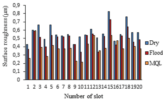
Figure 8: Surface-roughness results under different cooling/lubrication conditions
