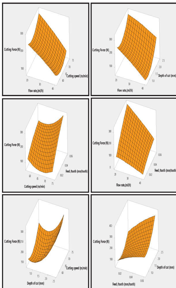
Figure 4: Cutting-force results for MQL condition
