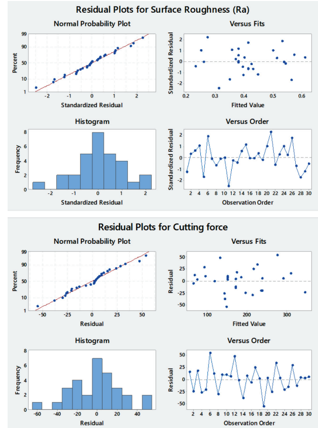
Figure 3: Residual analysis of MQL conditions
