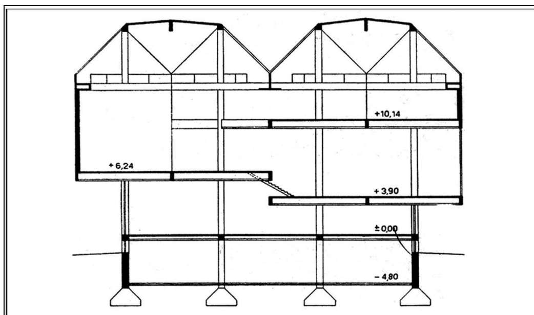
Figure 3.34. Longitudinal section of the Museum of Contemporary Art, Belgrade(Đorđević, 2017)
