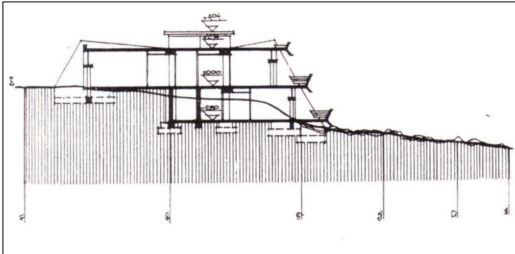
Figure 3.21. Cross section ( https://architectuul.com/architecture/hotel-podgorica )
