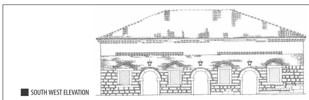
Figure 2.11. South west elevation of Military kitchen (Institute for the Protection of Cultural Monuments of the City of Belgrade. (n.d.)
