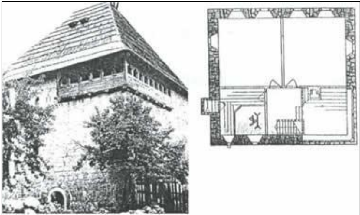
Figure 2.17. First floor plan, Ganica Kula(Hadžić, 2012)
