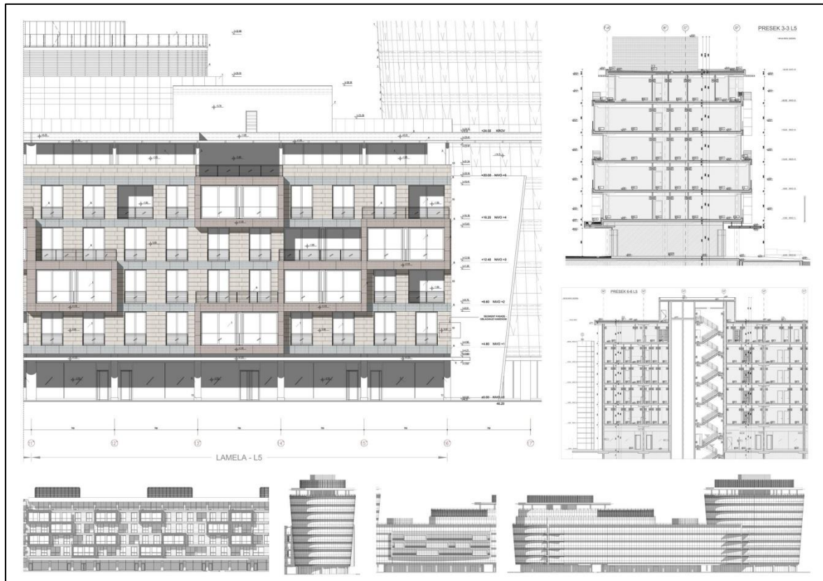
Figure 4.8. Facades and sections of the building (Real Estate Montenegro. (n.d.))
