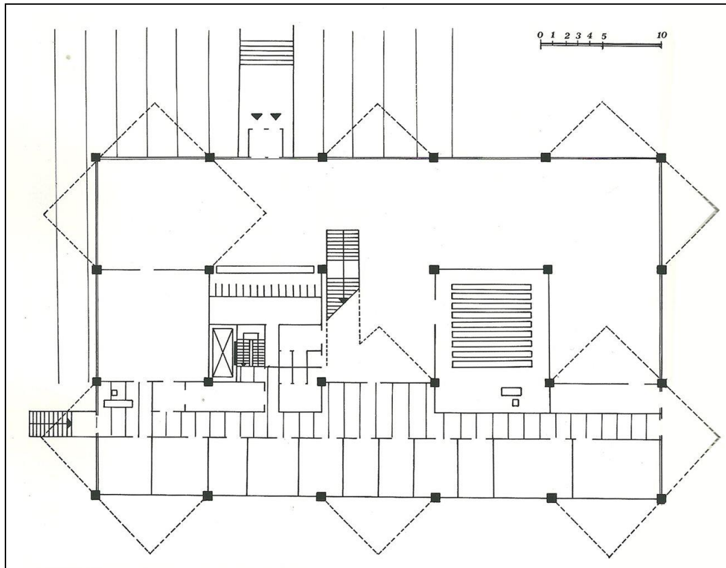
Figure 3.33. The first floor plan of the Museum of Contemporary Art, Belgrade(Đorđević, 2017)
