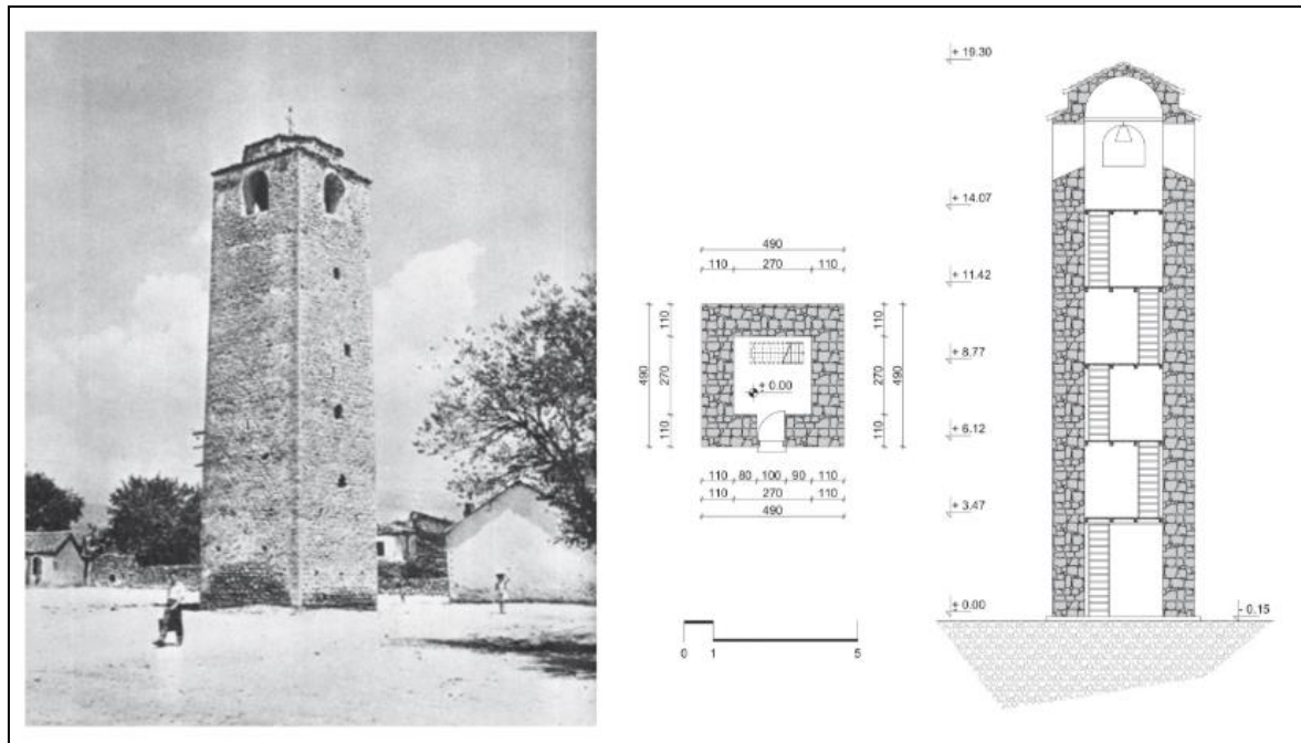
Figure 2.22. Plan and cross-section of the clock-tower in Stara Varoš-Podgorica 2018 (Drawing by R. Alihodžić)
