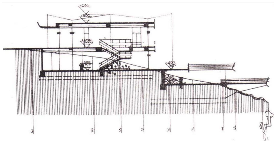
Figure 3.20. Longitudinal section B-B ( https://architectuul.com/architecture/hotel-podgorica )
