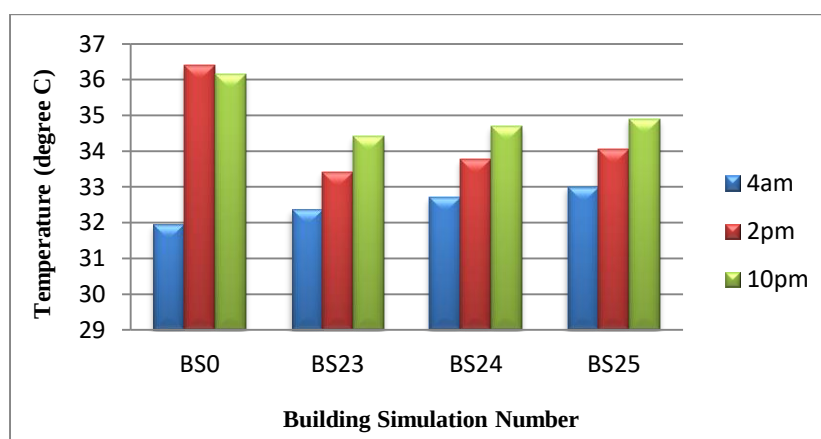
Figure 7.15. Changing the height of the wind catcher when the wind catcher dimension is (3 m * 3 m)
