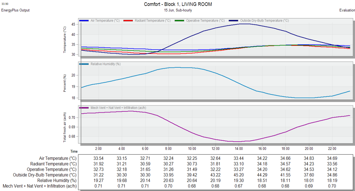
Figure 24. BS24 simulation charts
