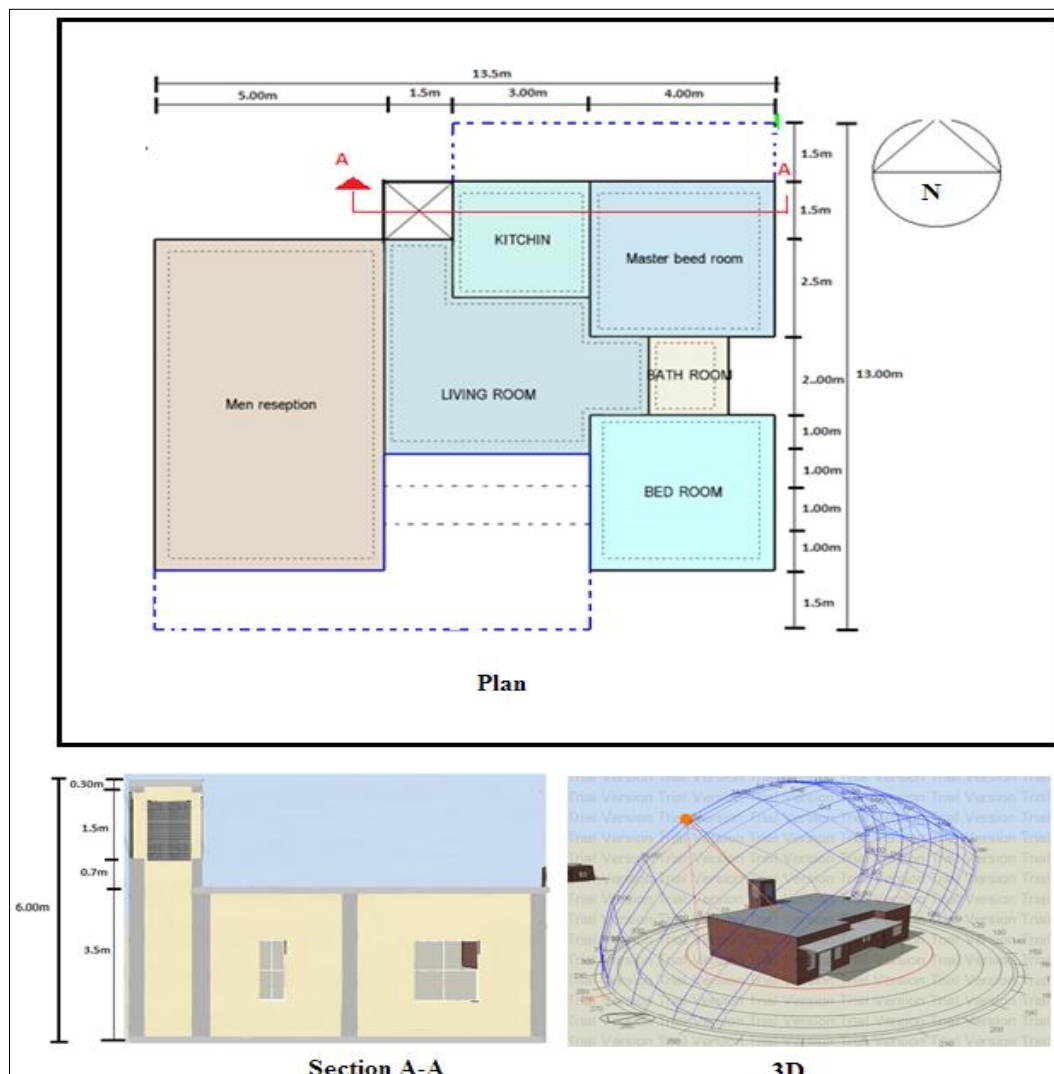
Figure 7.1. Design of the simulation traditional buildings' model
