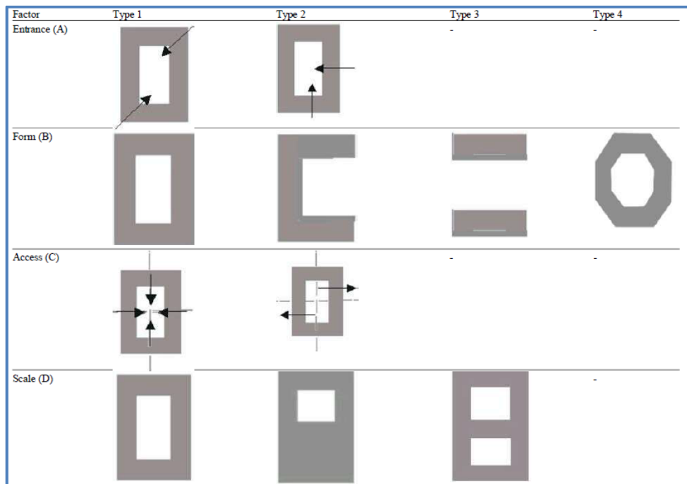
Figure 3.11. Different types of a central courtyard (Mahdavienejad et al., 2013)
