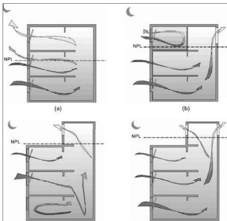
Figure 2.8. Different NBL locations with different opening designs room(Allard et al., 2012)
