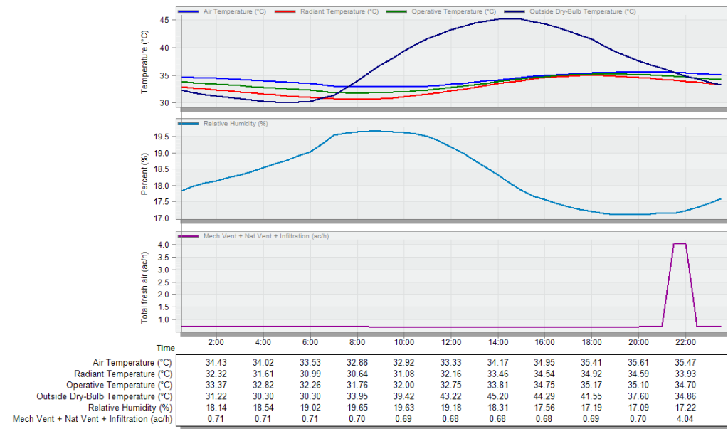
Figure 18. BS18 simulation charts
