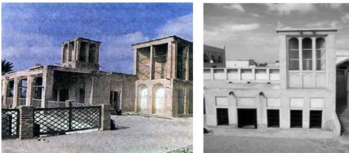
Figure 5.11. Wind-catcher in hot and humid area (Roaf, 2005)
