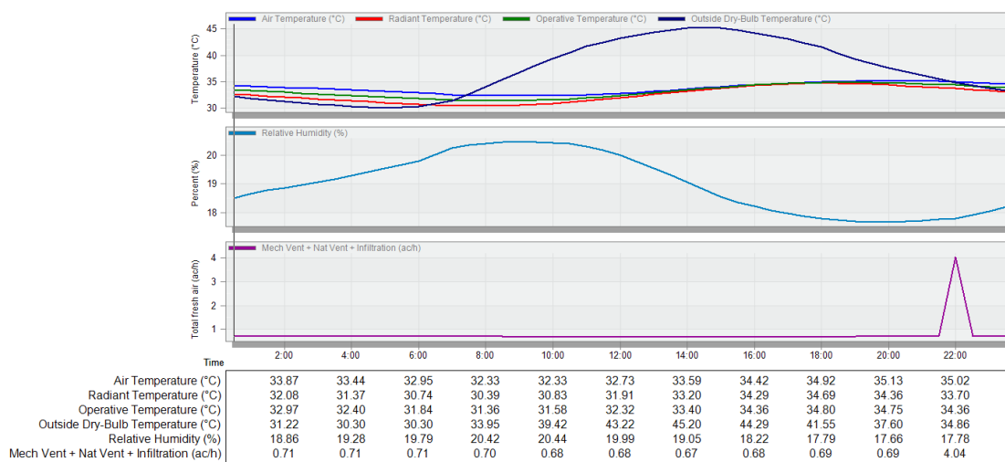
Figure 2. BS2 simulation charts
