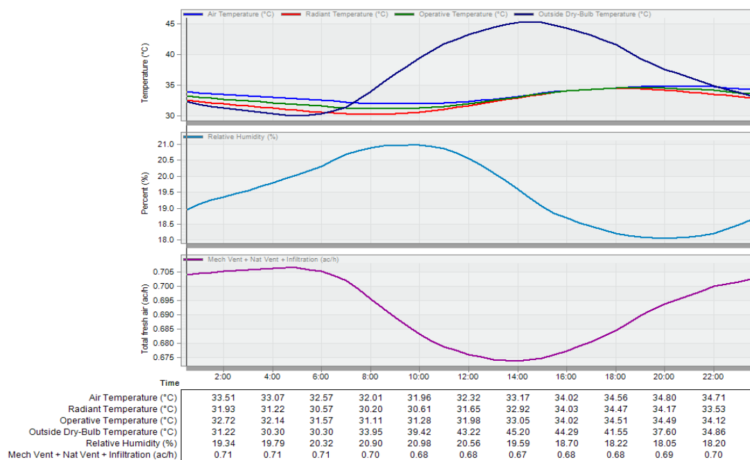
Figure 12. BS12 simulation charts
