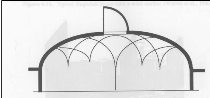
Figure 5.6 .Sketch of a typical wind catcher on top of a dome, Harat, Afghanistan (Mahyari, 1996)
